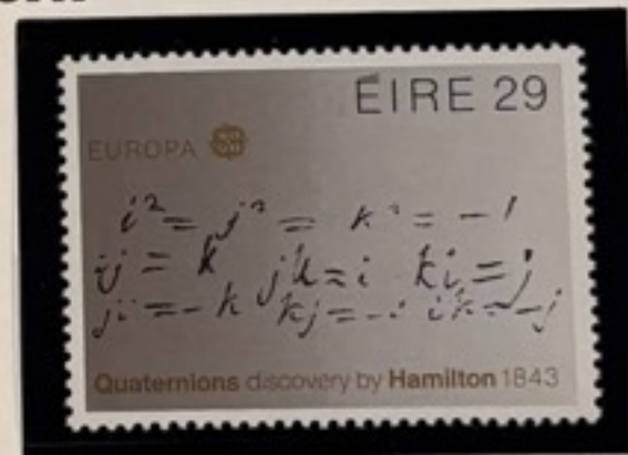
Equations (quaternions, multiplication law for complex numbers) by William Rowan Hamilton, 1843
